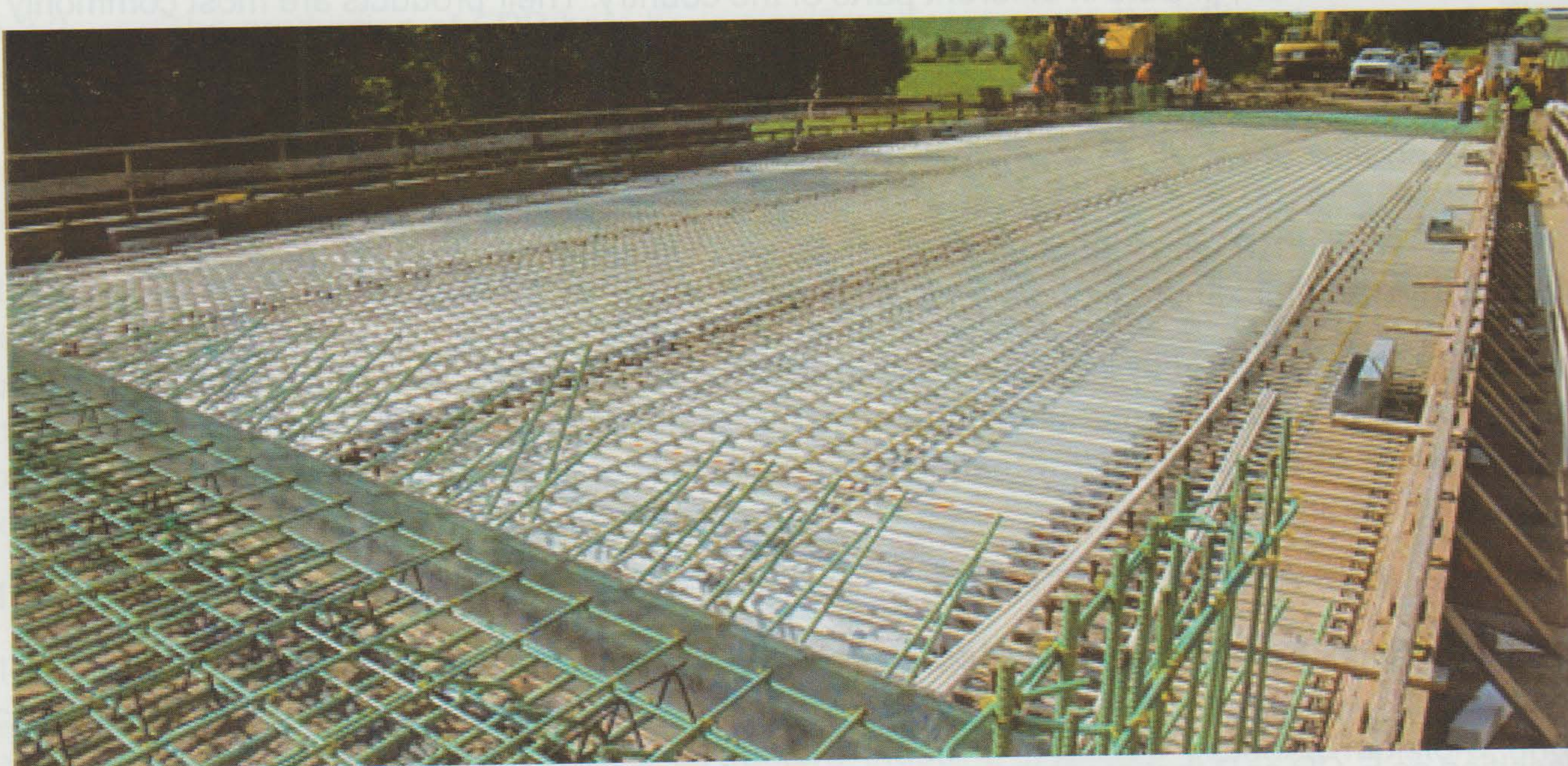
Fig. 2.1 Bridge Panel Construction Using GFRP Bars ( www.tuf-bar.com )
